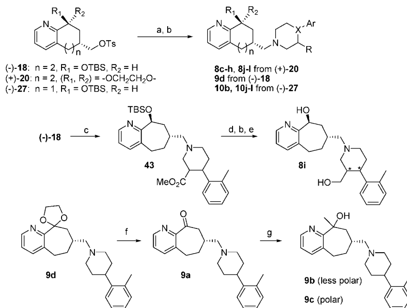
Scheme 6. Preparation of Final Products 8c–l , 9a–d , 10b , and 10j–l a
