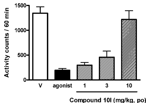
Figure 3. In vivo locomotor test by oral treatment of compound 10i at 1, 3, and 10 mg/kg.
