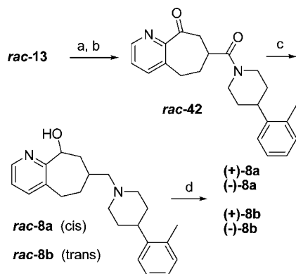
Scheme 5. Synthesis of 8a and 8b a
