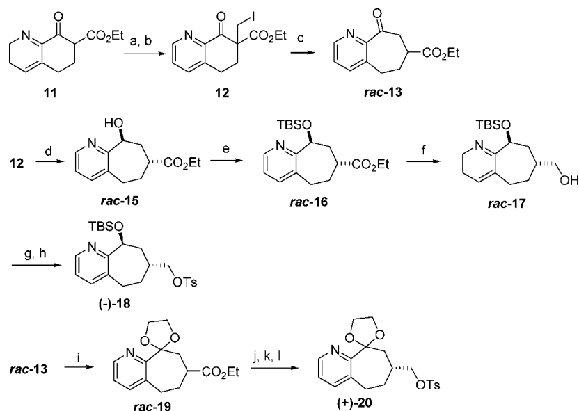
Scheme 1. Synthesis of Key Intermediates rac -13, (–)-18, and (+)-20 a
