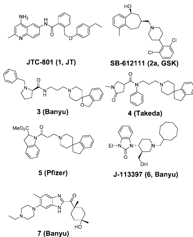
Figure 1. Reported ORL1 antagonists.
