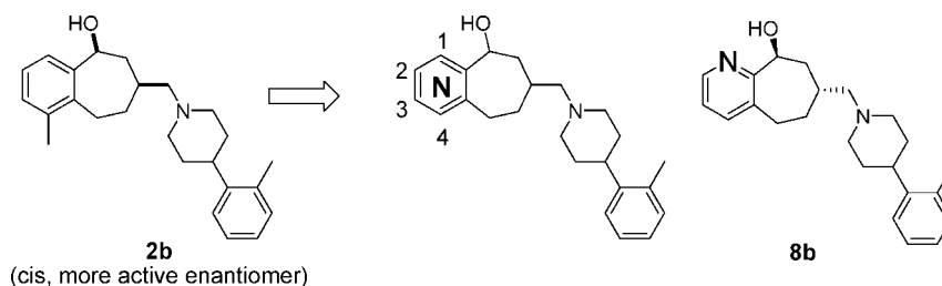
Figure 2. Incorporation of nitrogen atom in benzosuberonyl moiety.
