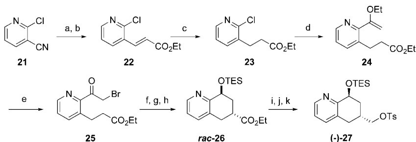
Scheme 2. Synthesis of Key Intermediate (–)-27 a
